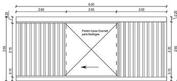
VISTA FRONTAL Esc: 1/40
